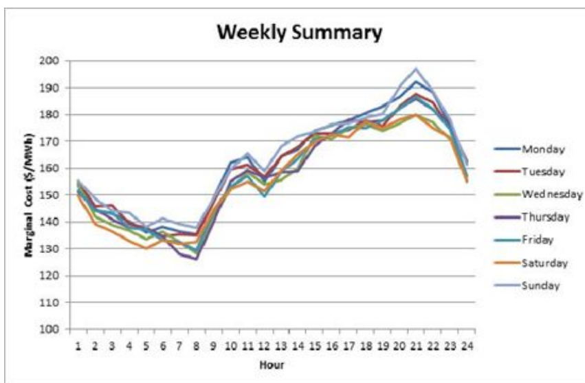
Figure 4 Weekly Marginal Electric Costs Assuming Cabras Unit 3 is Offline
